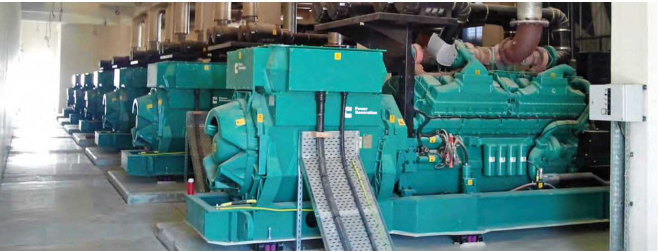
6 nos. 2500 kVA, 11 kV generator with automatic load management and with bump less restoration at RGO complex
